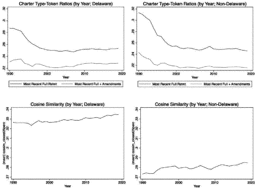
Figure 7: Mean Type-Token Ratio and 25%-Nearest-Neighbor Cosine Similarity
